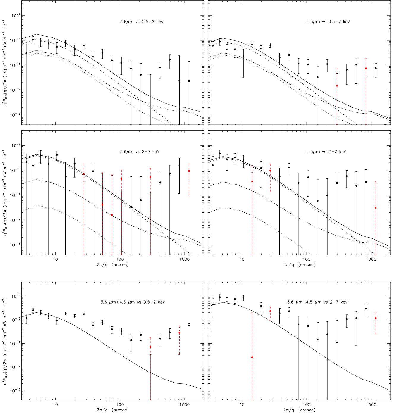
FIG. 2.— Combined CIB-CXB cross-power spectra ( black filled circles ). Top, center panels : 3.6 \mu\text{m} vs. 0.5\text{--}2 \text{ keV} , 4.5 \mu\text{m} vs. 0.5\text{--}2 \text{ keV} , 3.6 \mu\text{m} vs. 2\text{--}7 \text{ keV} and 4.5 \mu\text{m} vs. 2\text{--}7 \text{ keV} . We over-plot our reconstruction of known z < 6 populations: dashed line for AGN, dot-dashed line for star-forming galaxies, dotted lines for hot gas in clusters and solid lines for the sum. Bottom panels : Cross-power of combined CIB ( 3.6+4.5 \mu\text{m} ) vs. ( left ) soft X-ray ( 0.5\text{--}2 \text{ keV} ) and ( right ) hard X-ray ( 2\text{--}7 \text{ keV} ) bands.
